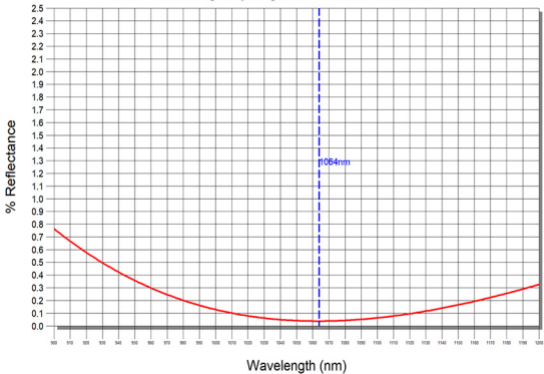
A1000: Single Layer MgF2 on Nd:YAG for 1064nm
