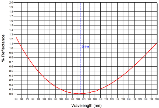
23 Layer Quasi-Rugate AR 1064nm on Fused Silica (Batch# 19-135)
